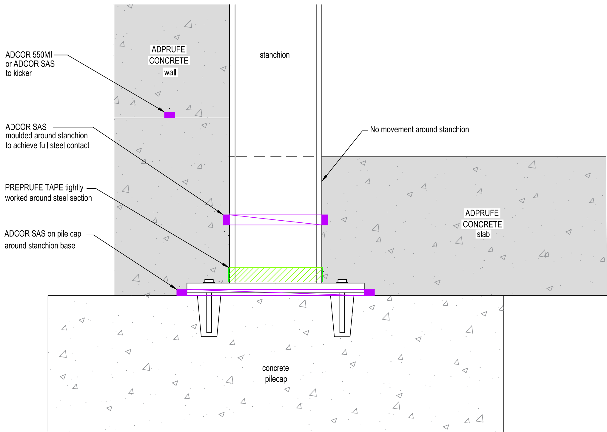
SLAB-WALL KICKER AT STANCHION INTERFACE - SECTION
