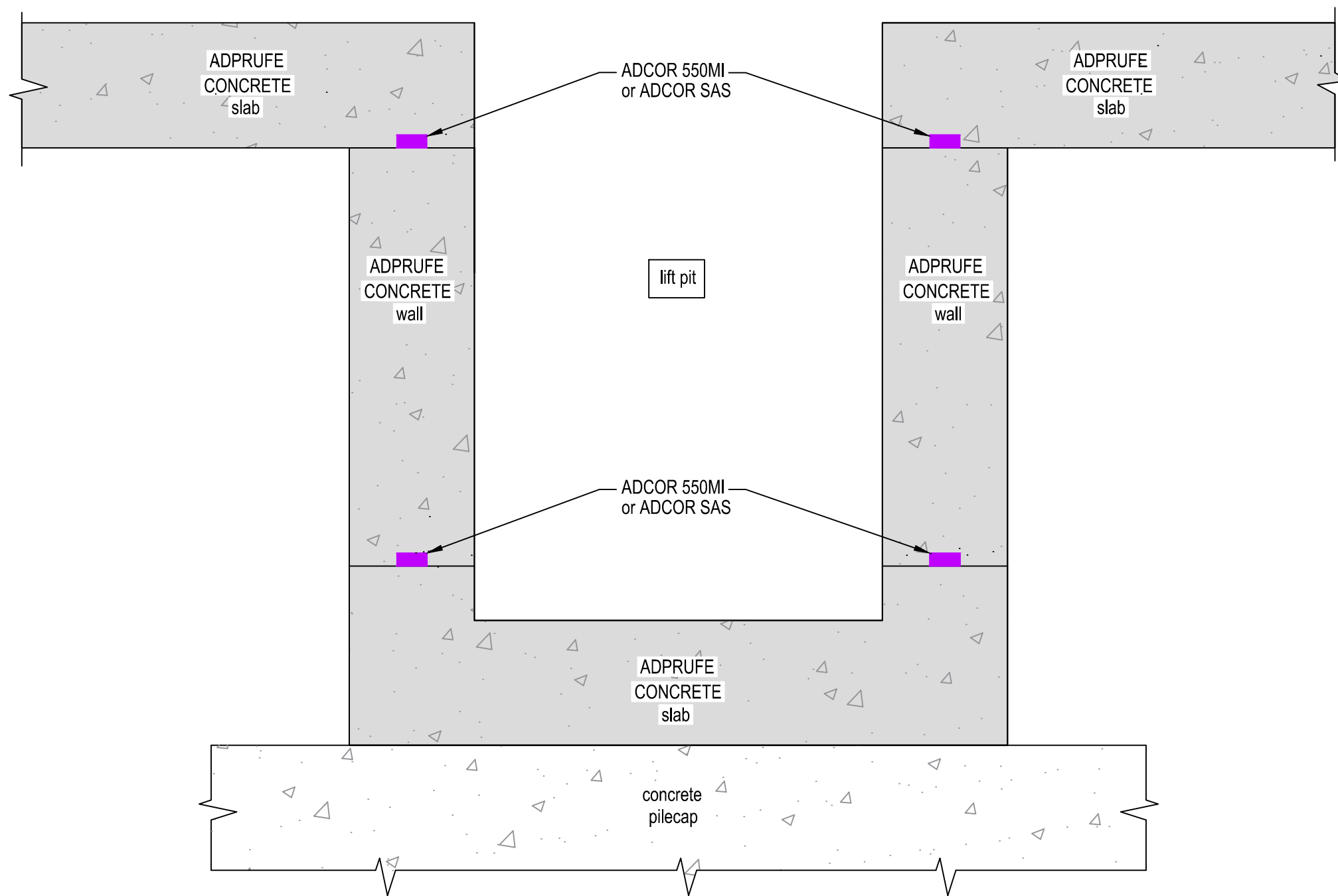
LIFT PIT DETAIL SECTION
