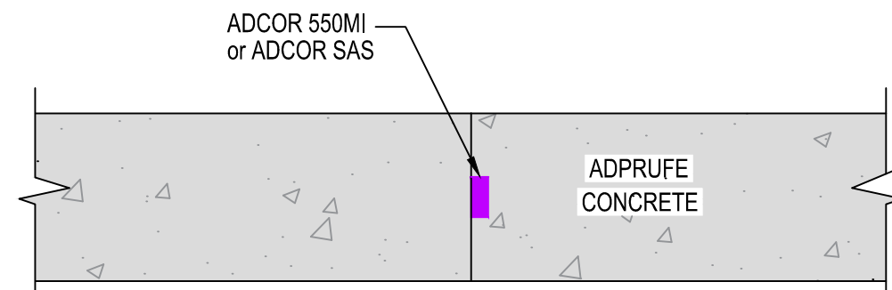
WALL / SLAB CONSTRUCTION JOINT DETAIL PLAN / SECTION
