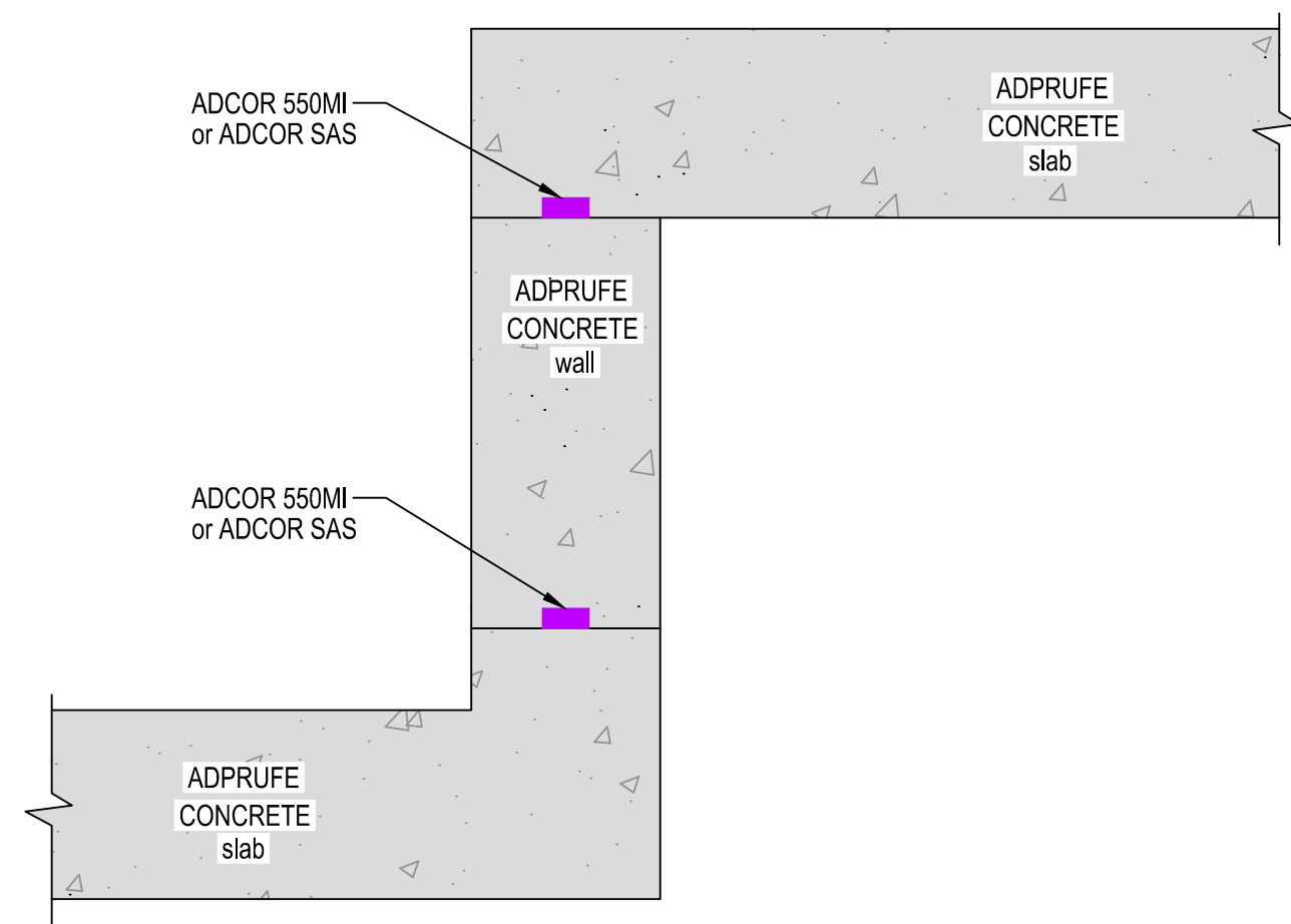
KICKER DETAIL SECTION
