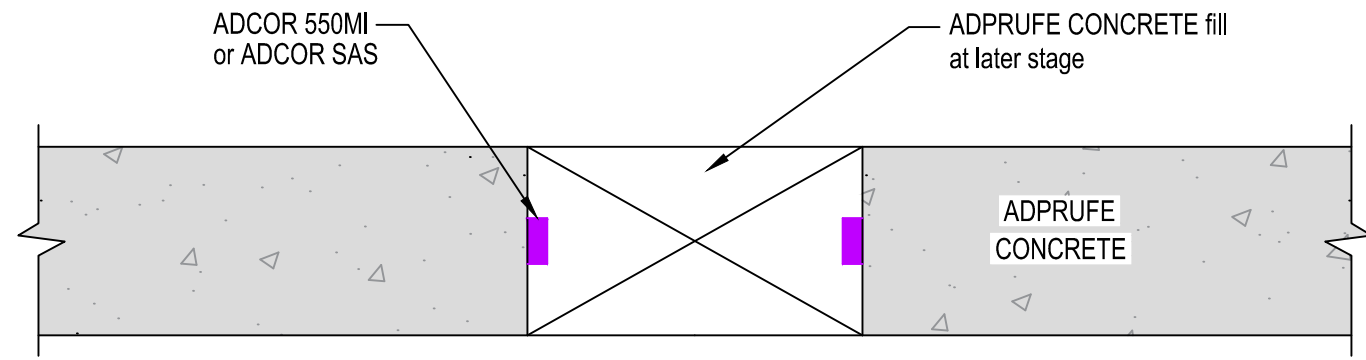
BOX OUT DETAIL SECTION / PLAN
